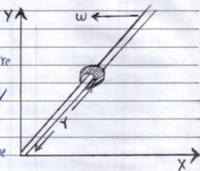
Fig: A Bead sliding on uniformly rotating wire
